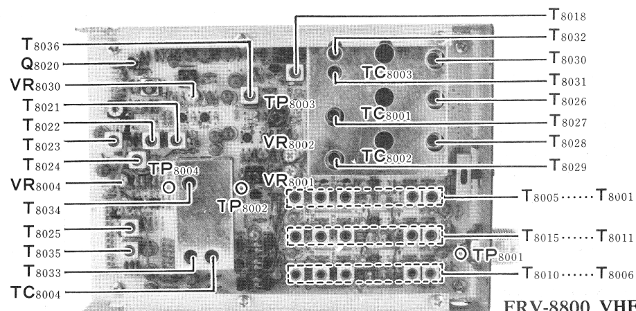
MAIN UNIT ALIGNMENT POINTS (BOTTOM VIEW)
