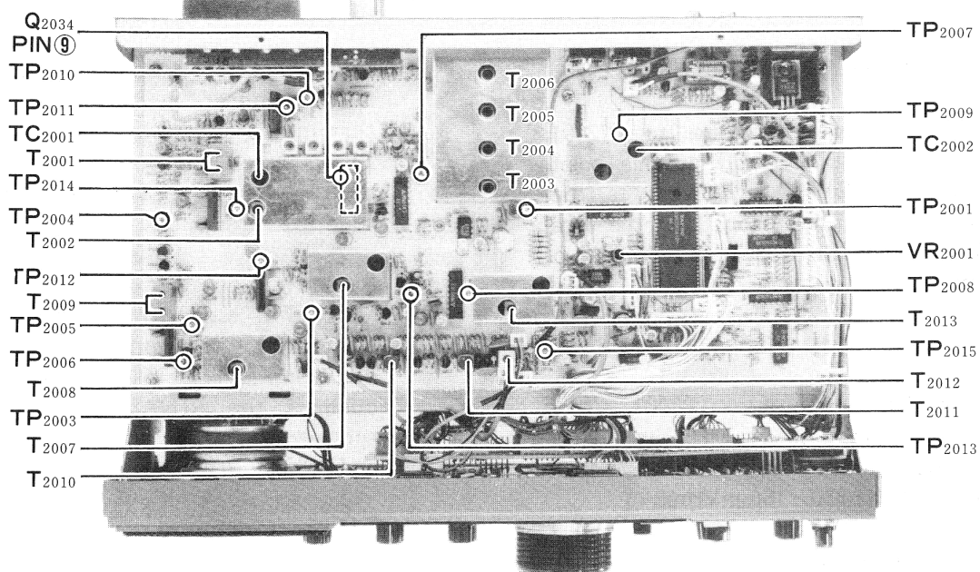
PLL UNIT ALIGNMENT POINTS (TOP VIEW)
