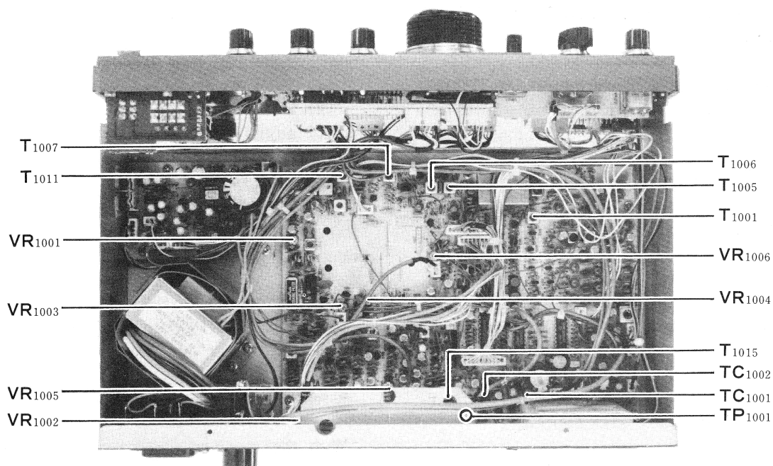
MAIN UNIT ALIGNMENT POINTS (BOTTOM VIEW)
